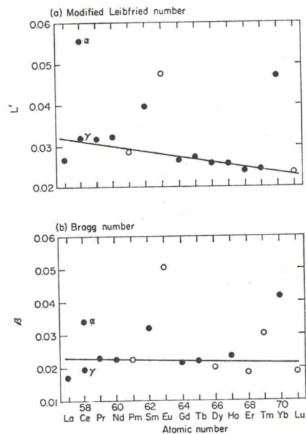
FIG. 28. (a) The modified Leibfried number of the rare-earth metals. (b) The Bragg number of the rare-earth metals. Open points are estimated data.
